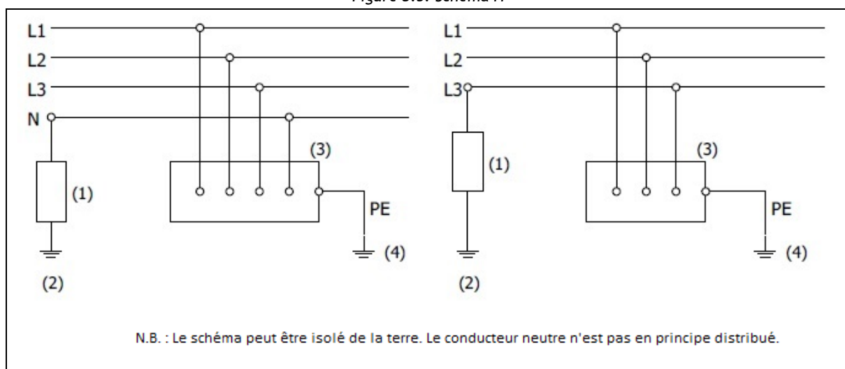
Figure 3.5. Schéma IT
