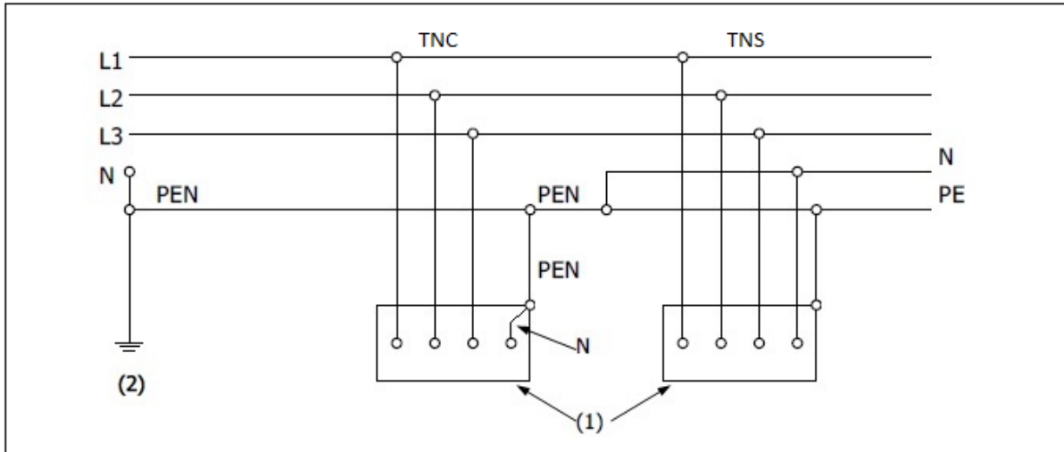
Figure 2.3. Schéma TN-C-S
