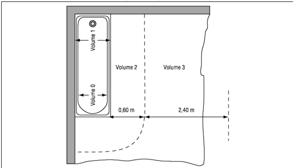
Figure 7.1. Baignoire
