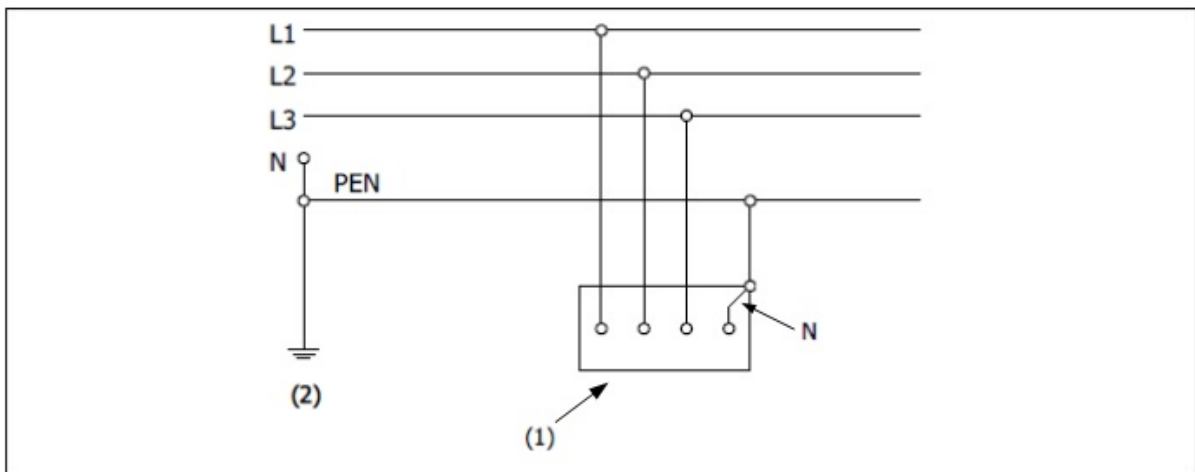
Figure 2.2. Schéma TN-C
