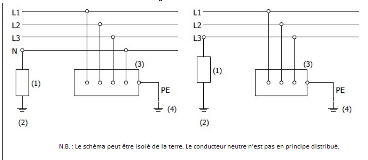
Figure 2.5. Schéma IT
