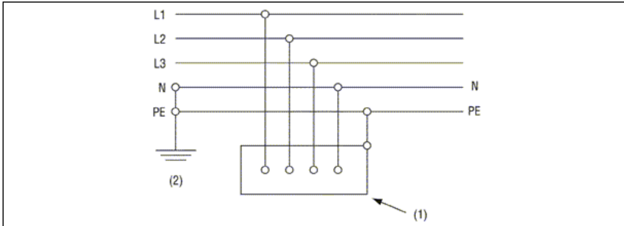
Figure 2.1. Schéma TN-S
