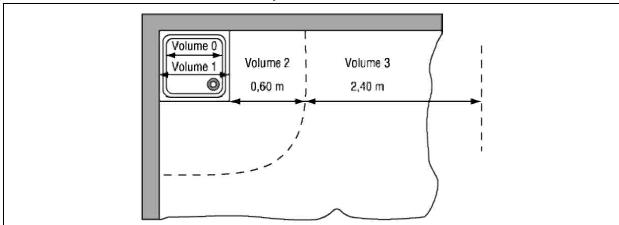
Figure 7.3. Douche
