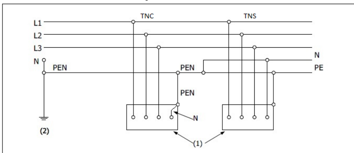
Figure 3.3. Schéma TN-C-S
